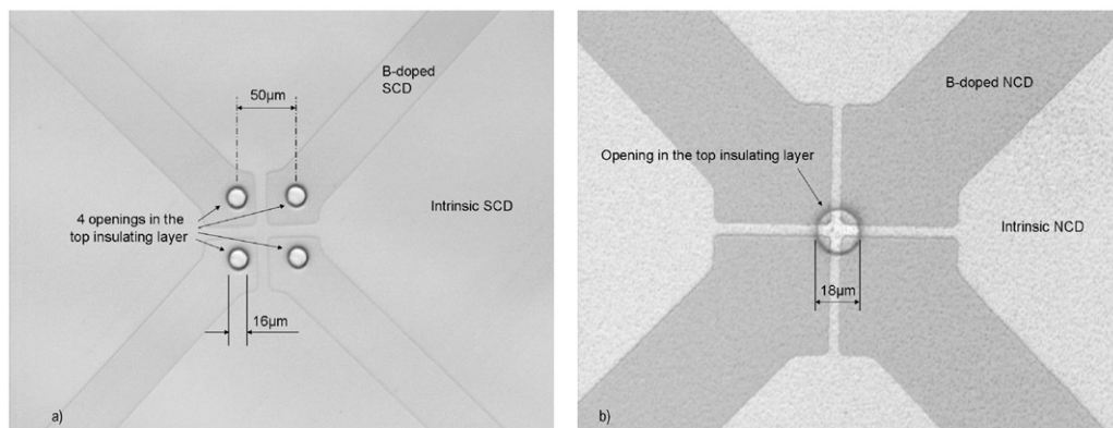
Figure 2. (a) SCD device with four separated circular apertures, having 16\ \mu\text{m} diameter and 50\ \mu\text{m} pitch. (b) NCD quadrupole on sapphire substrate with a single aperture 18\ \mu\text{m} in diameter. Due to limited precision in the alignment of the lithographic mask, the contact area is slightly asymmetric, leading to different signal-to-noise ratios among the electrodes.
